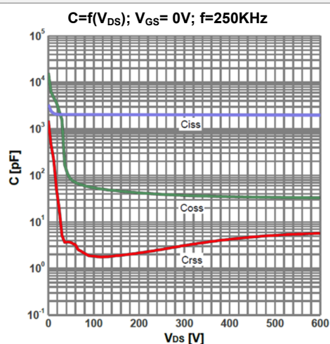
Figure 12. Typ. Capacitances
