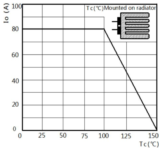
Derating Curve For Output Rectified Current
