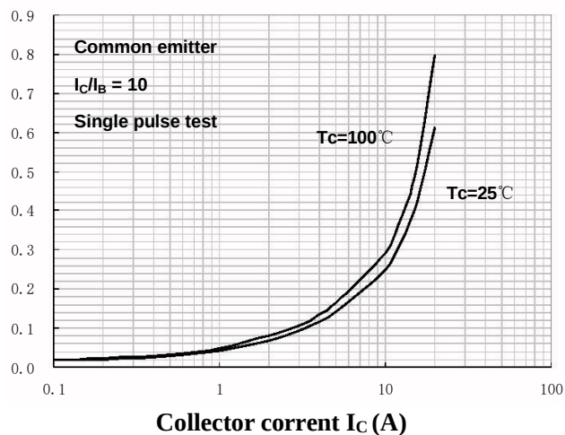
Saturation Voltage
