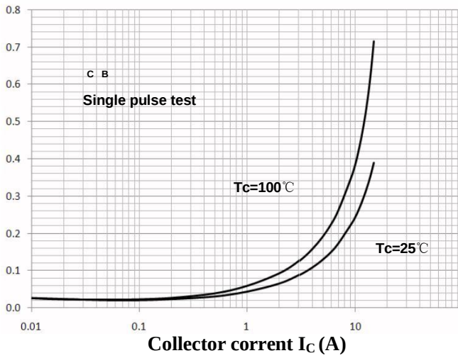
Saturation Voltage
