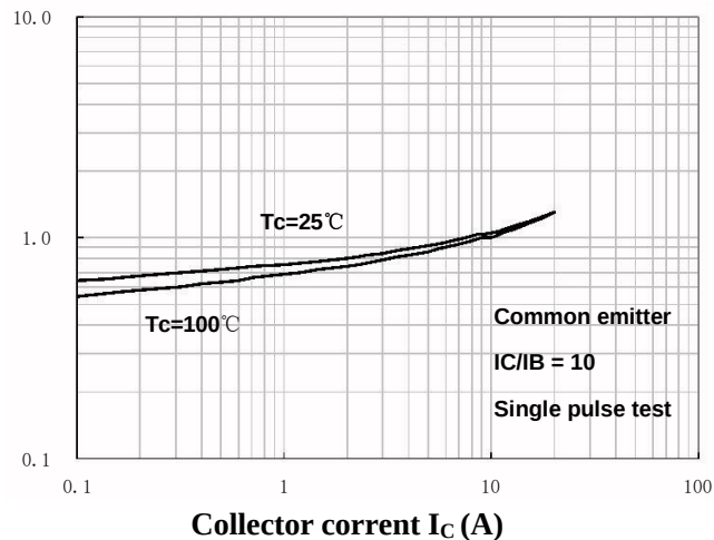
Base-Emitter Voltage
