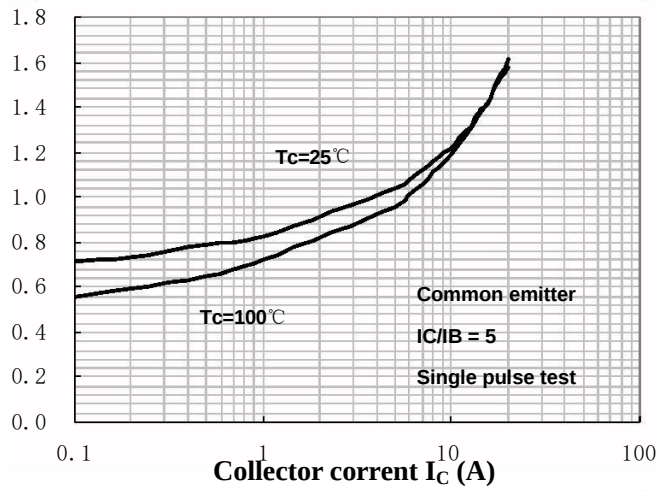
Saturation Voltage
