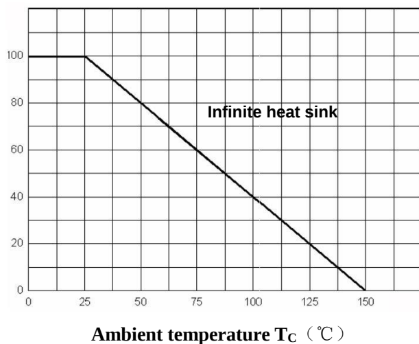
Power Derating
