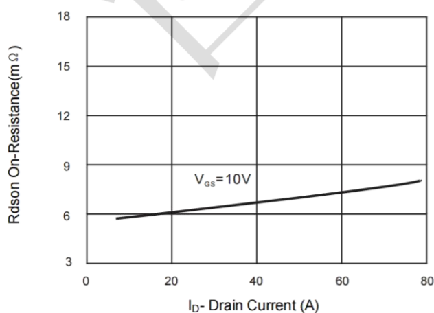
Fig. 5-Rdson- Drain Current
