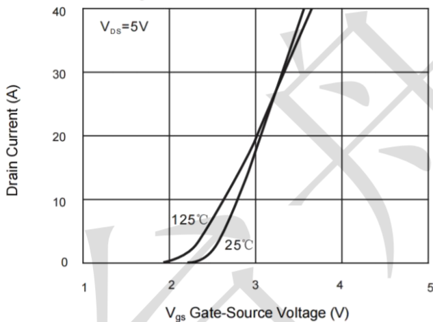
Fig. 3-Transfer Characteristics
