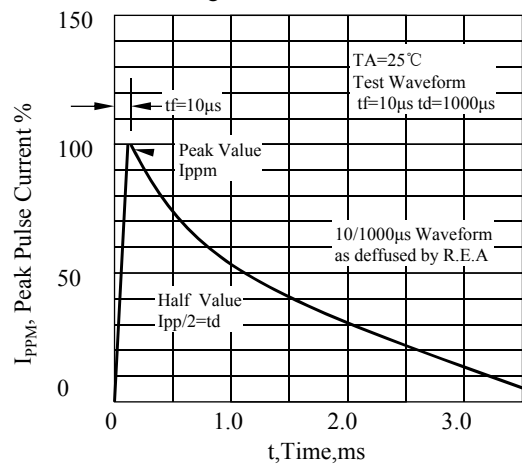
Fig. 1-Pulse Waveform
