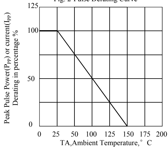
Fig. 2-Pulse Derating Curve
