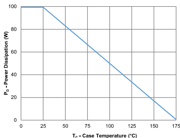
Figure 10: Power Derating
