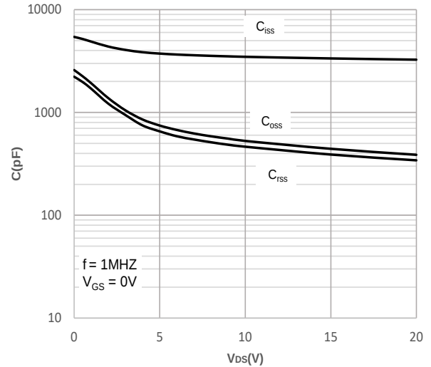
Figure 6: Capacitance Characteristics
