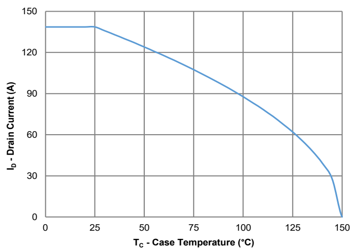
Figure 11: Current Derating
