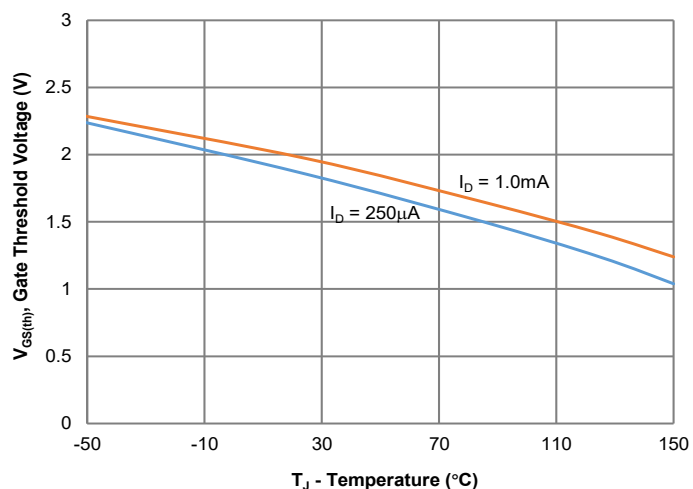
Figure 7: Gate Threshold Variation vs. Junction Temperature
