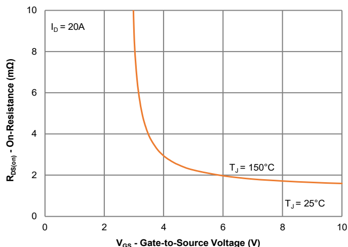
Figure 3: On-Resistance vs. Gate-Source Voltage
