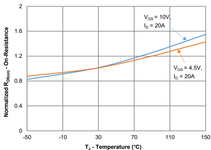
Figure 5: On-Resistance vs. Junction Temperature
