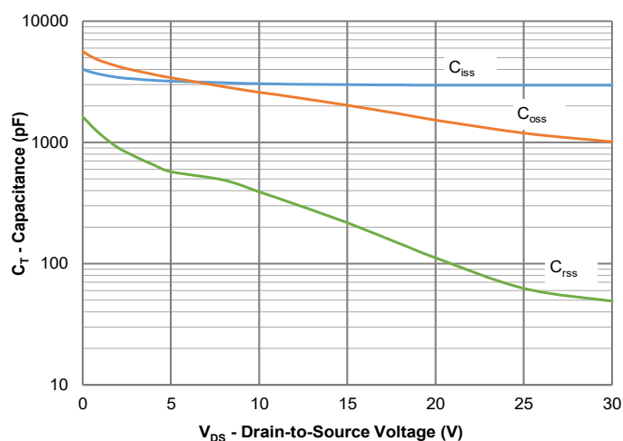
Figure 9: Capacitance Characteristics
