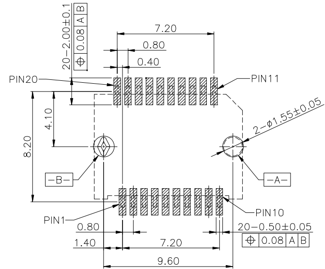
RECOMMENDED PCB LAYOUT(TOP VIEW) (ALL TOLERANCES ARE ±0.05)
