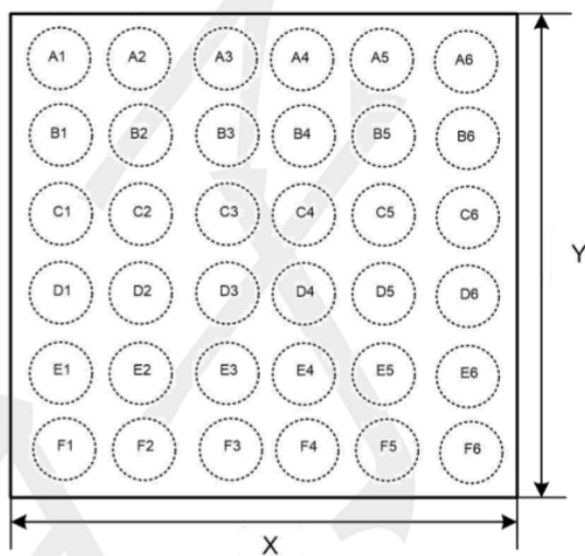
Top-Through View
