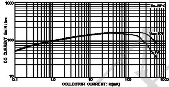
Fig.3 DC current gain vs. collector current (I)
