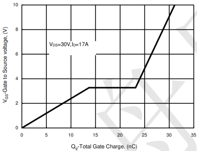
FIG.9- Gate Charge
