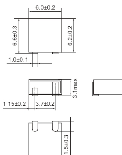
CDBB Series
