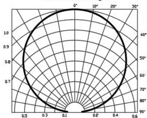
Radiation angle
