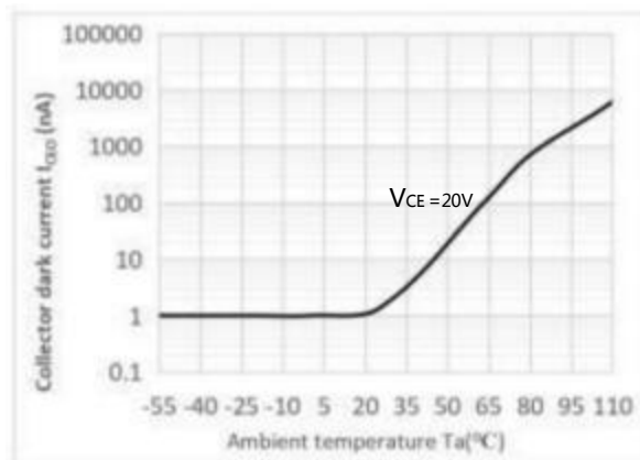
Fig.2 Collector Dark Current vs Ambient Temperature
