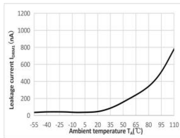
Fig.6 Leakage current vs Ambient temperature
