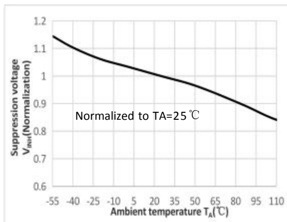
Fig.8 Suppression voltage vs Ambient temperature
