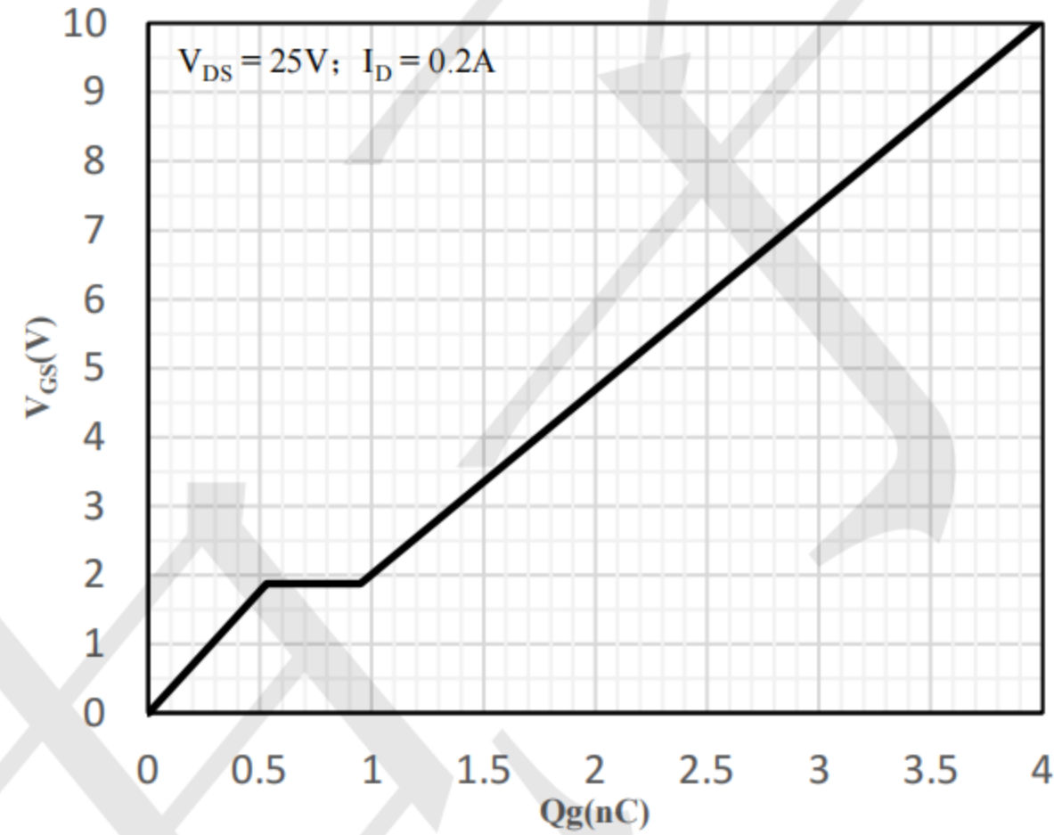
Fig 8 Gate-Charge Characteristics
