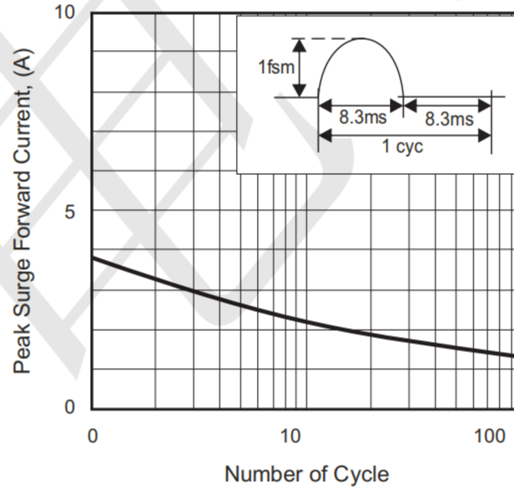
Fig.4 - IFSM-Cycle Characteristics
