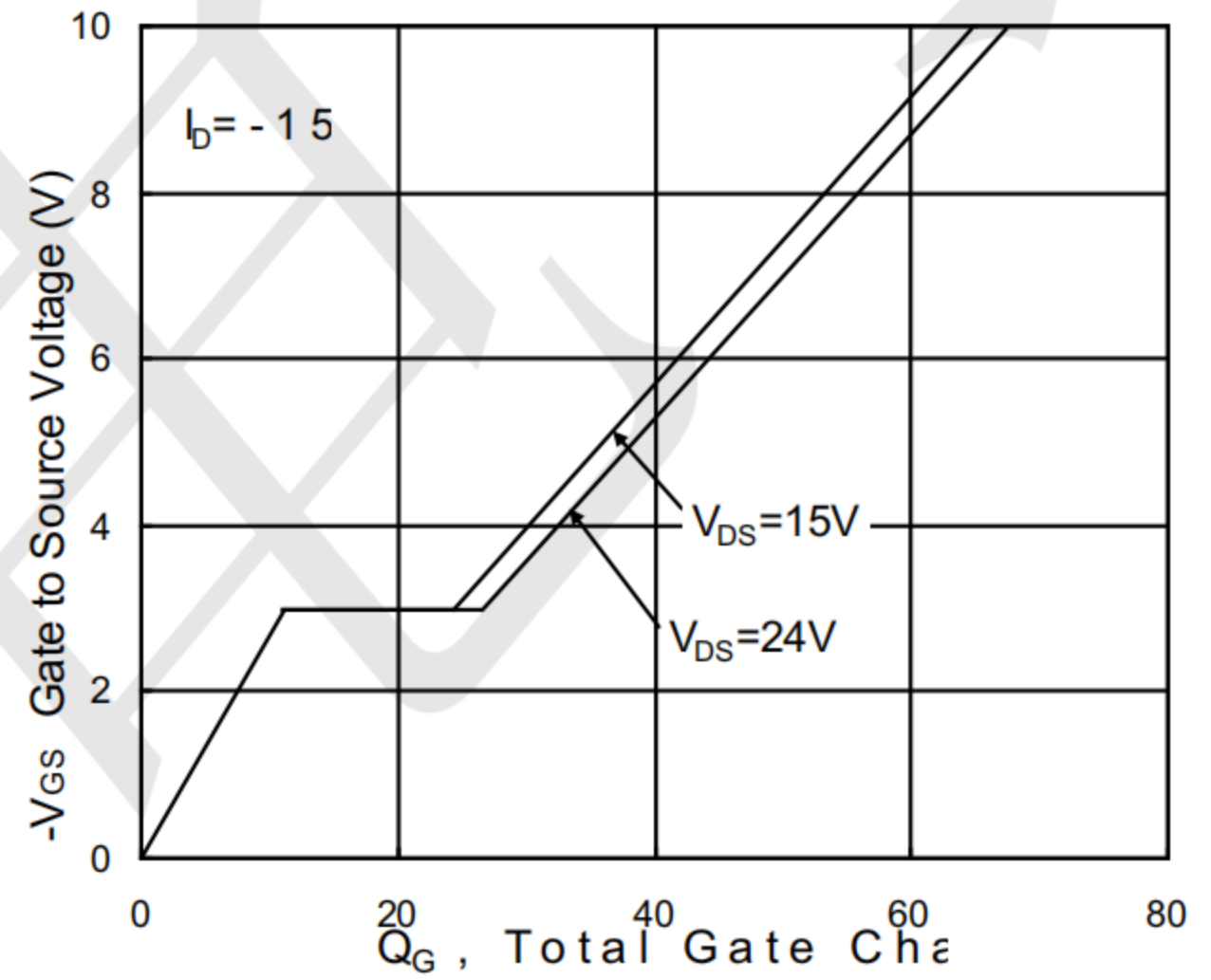
Fig.4 Gate-Charge Characteristics
