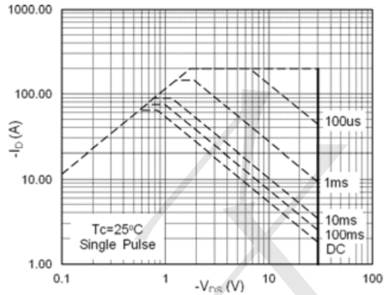
Fig.8 Safe Operating Area
