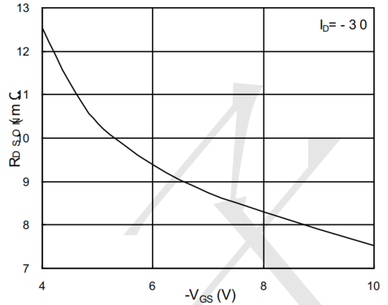
Fig.2 On-Resistance v.s Gate-Source
