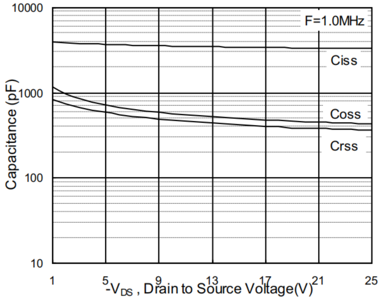
Fig.7 Capacitance
