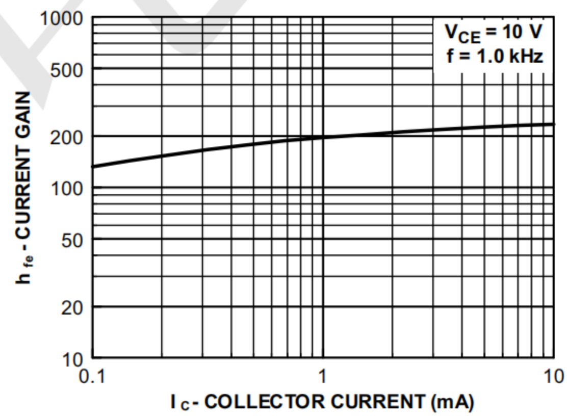
Figure 15. Current Gain
