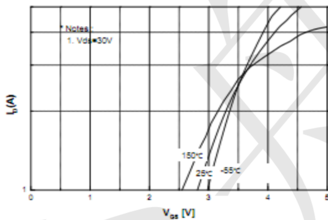
Fig.5 Transfer Characteristics
