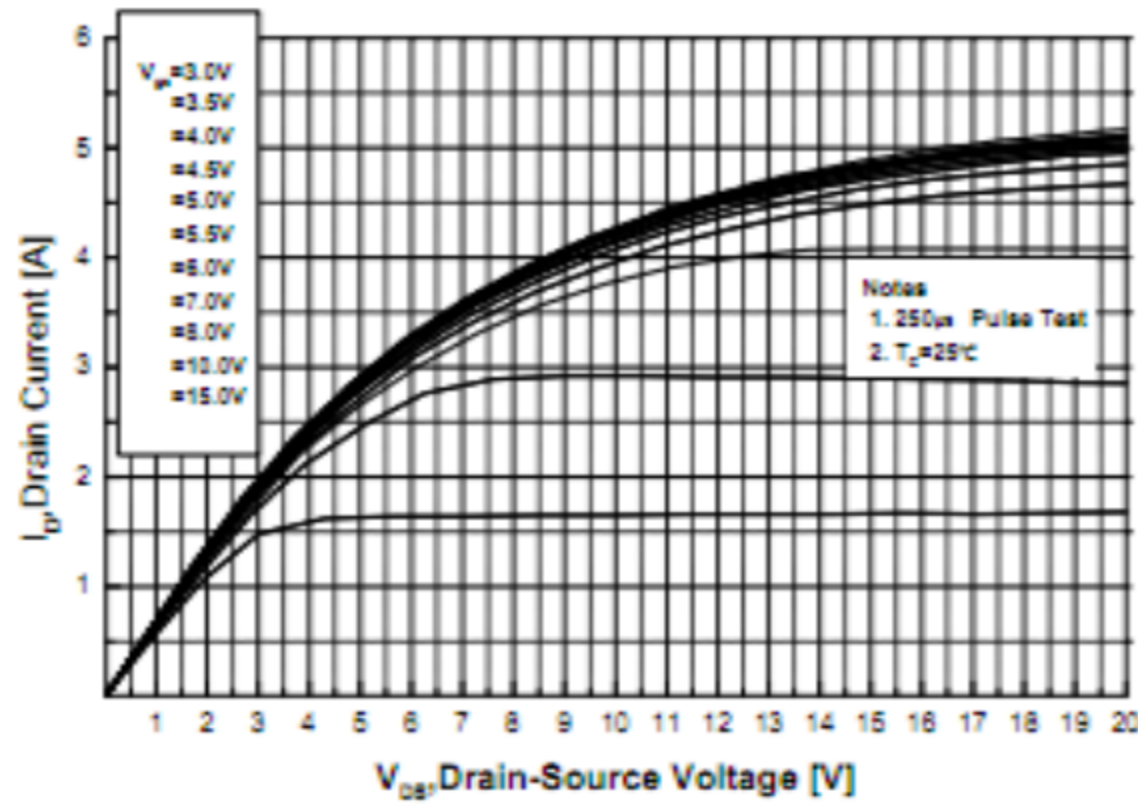
Fig.1 On-Region Characteristics
