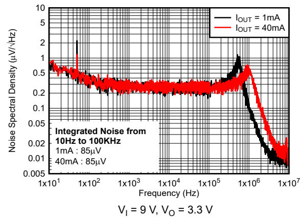
图 6-20. Noise Spectral Density vs Frequency and I_O for New Chip
