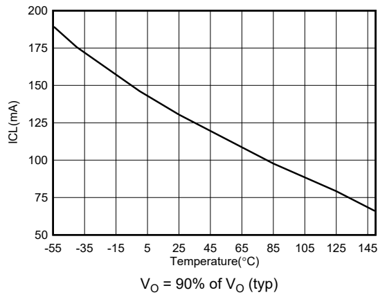
图 6-19. I_{CL} vs Temperature for New Chip
