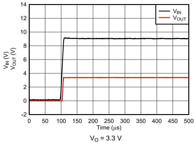
图 8-6. Start-Up With Fast V_I Ramp for New Chip
