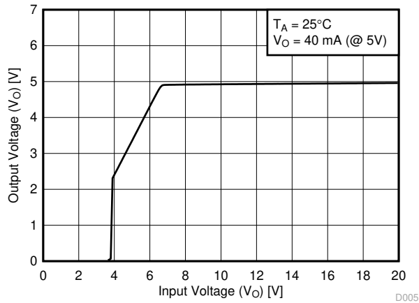
图 8-4. Output Voltage vs Input Voltage for Legacy Chip
