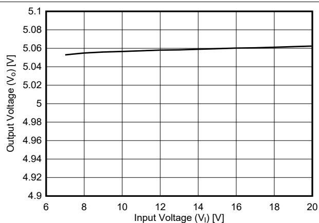
图 6-8. Line Regulation at I_O = 1\text{ mA} for New Chip at T_J = 25^\circ\text{C}
