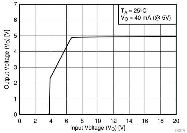
图 8-5. Output Voltage vs Input Voltage for New Chip
