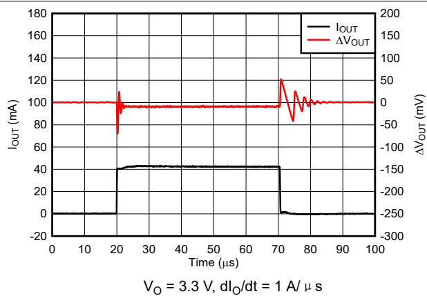
图 8-8. Load Transient Behavior for New Chip
