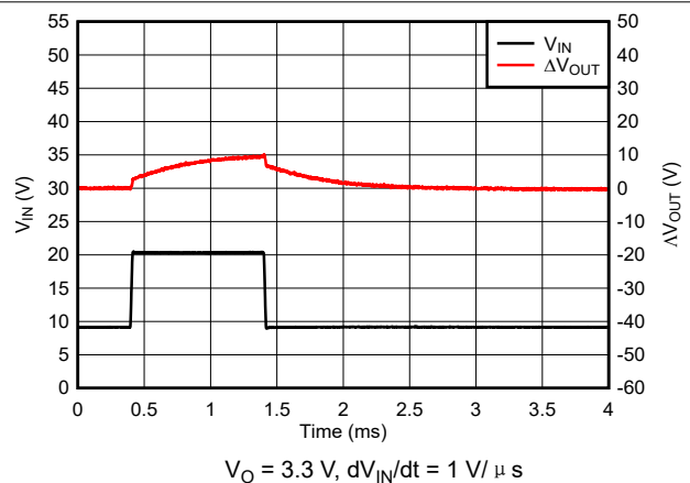
图 8-9. Line Transient Behavior for New Chip
