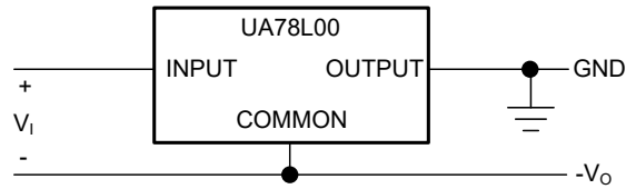
图 8-10. Positive Regulator in Negative Configuration ( V_I Must Float)
