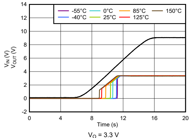
图 8-7. Start-Up With Slow V_I Ramp Across Temperature for New Chip
