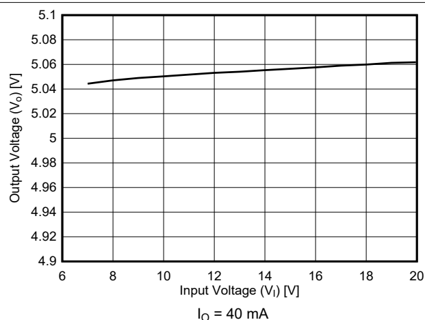
图 6-7. Line Regulation at I_O = 40\text{ mA} for New Chip at T_J = 25^\circ\text{C}
