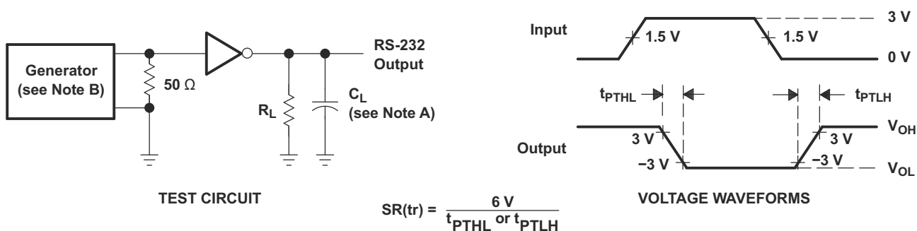
图 6-1. Driver Slew Rate
