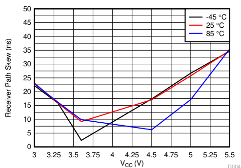
图 5-7. Receiver Path Skew ( |t_{pHL} - t_{pLH}| ) (RGT Package)
