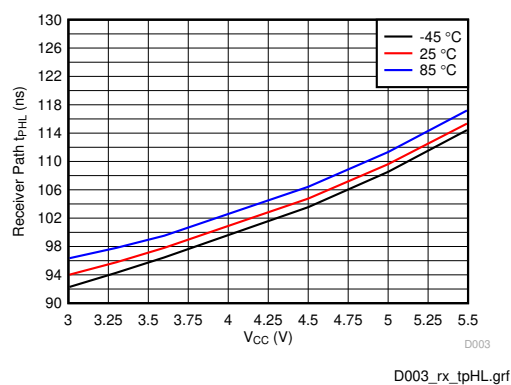
图 5-6. Receiver Path High-to-Low Propagation Delay (RGT Package)
