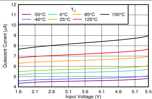
图 5-37. I_{GND} vs V_{IN} in the Dropout Region
