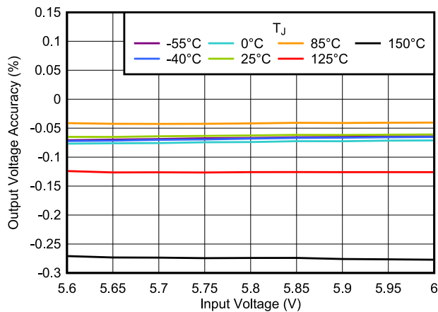
图 5-22. Output Voltage Accuracy vs V_{IN}
