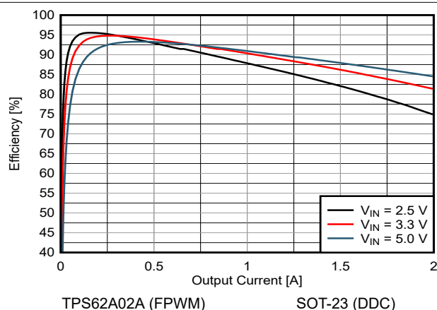
图 8-19. 1.8V Output Efficiency
