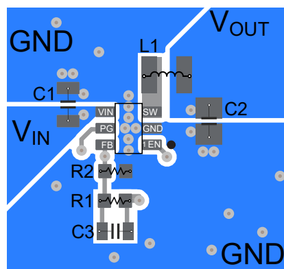
图 8-25. TPS62A0x (SOT23-6) PCB Layout Recommendation
