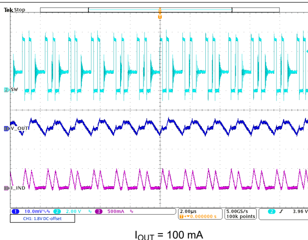
图 8-21. Power Save Mode Operation
