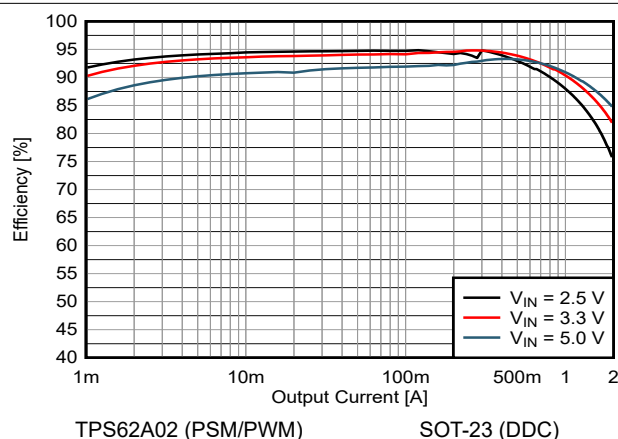
图 8-18. 1.8V Output Efficiency
