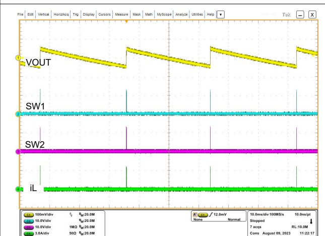
图 8-5. Switching Waveforms in V_{IN} = 12\text{ V} , V_{OUT} = 12\text{ V} , I_O = 0\text{ A} , PFM
