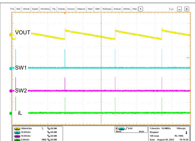
图 8-3. Switching Waveforms in V_{IN} = 16\text{ V} , V_{OUT} = 12\text{ V} , I_O = 0\text{ A} , PFM
