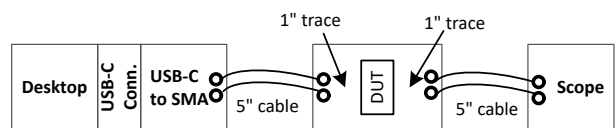
图 7-10. 10Gbps USB Compliance Setup - with TMUXHS4446
