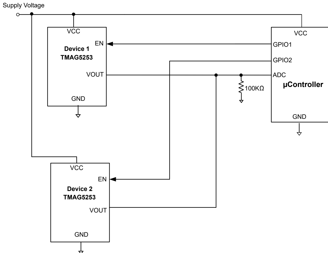
图 9-1. Multiple Sensors With Shared Output
