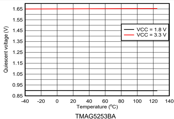
图 6-12. TMAG5253BA Quiescent Voltage vs Temperature
