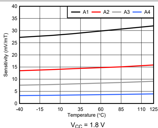
图 6-8. TMAG5253BA Sensitivity vs Temperature
