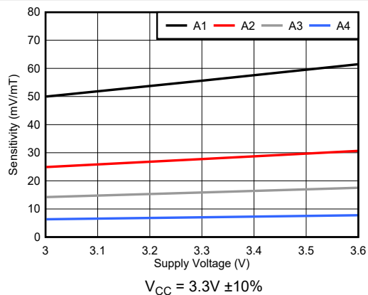
图 6-11. TMAG5253BA Sensitivity vs Supply Voltage
