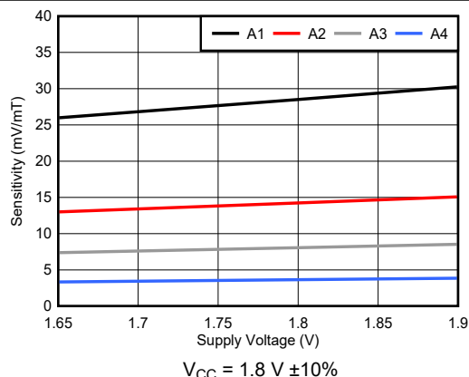
图 6-10. TMAG5253BA Sensitivity vs Supply Voltage
