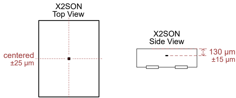
图 8-3. Hall Element Location
