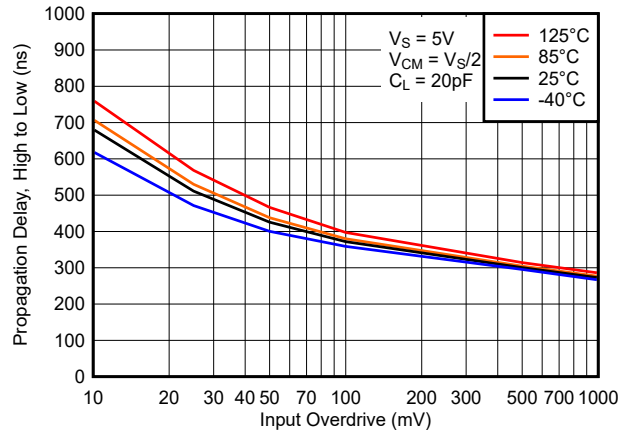
图 6-13. Propagation Delay, High to Low, 5V
