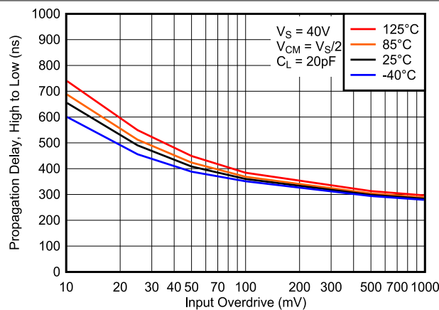
图 6-17. Propagation Delay, High to Low, 40V
