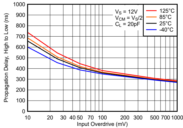
图 6-15. Propagation Delay, High to Low, 12V
