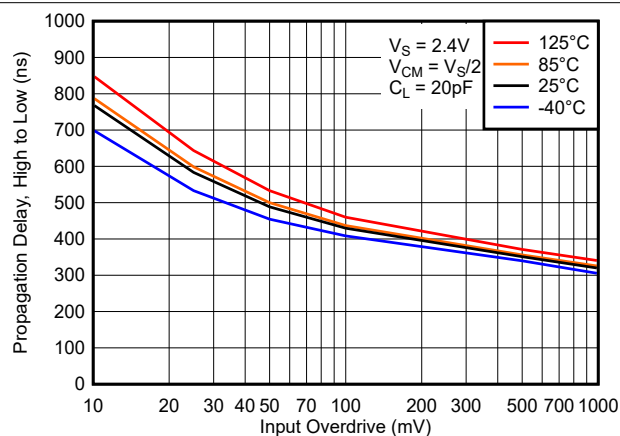
图 6-11. Propagation Delay, High to Low, 2.4V
