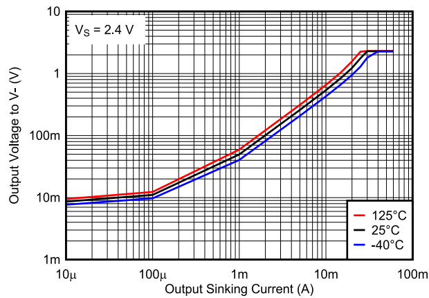
图 6-3. Output Voltage vs. Output Sinking Current, 2.4V
