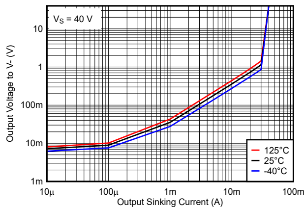
图 6-9. Output Voltage vs. Output Sinking Current, 40V
