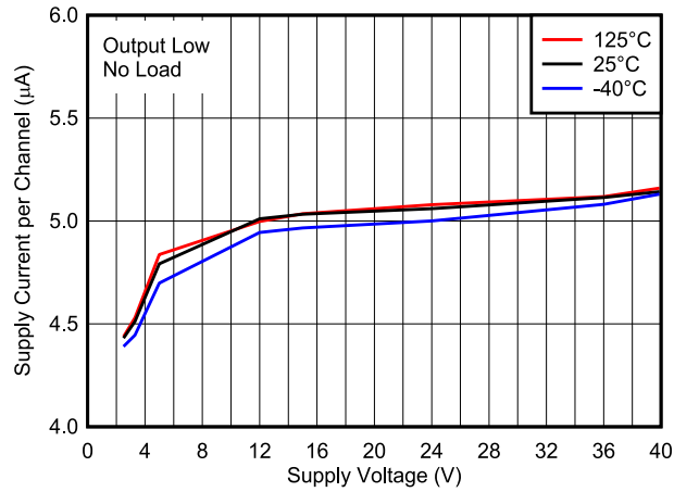
图 6-1. Supply Current per Channel vs. Supply Voltage, Output Low
