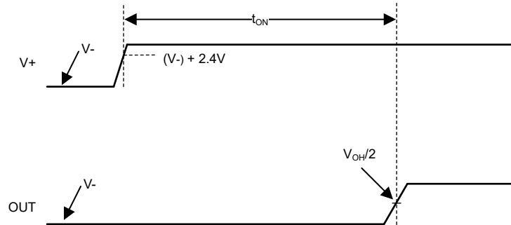
图 7-3. Power-On Reset Timing Diagram
