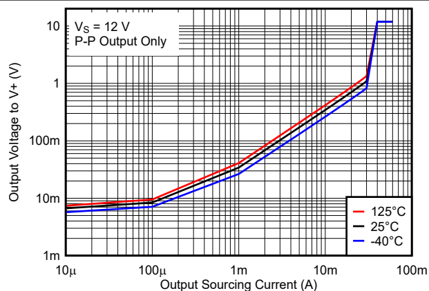
图 6-8. Output Voltage vs. Output Sourcing Current, 12V
