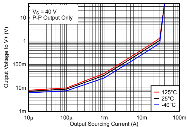
图 6-10. Output Voltage vs. Output Sourcing Current, 40V
