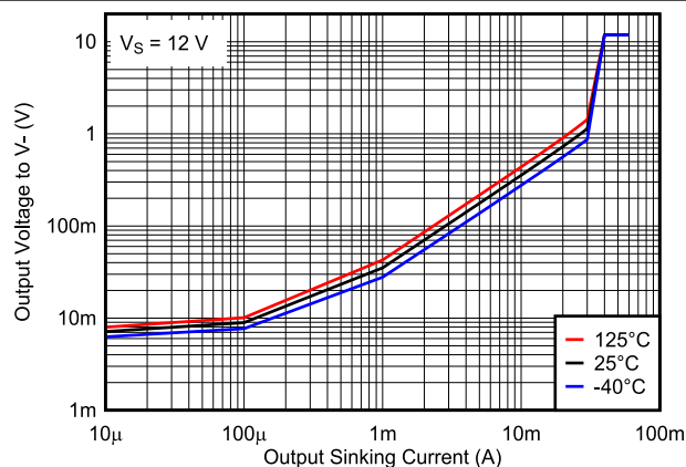
图 6-7. Output Voltage vs. Output Sinking Current, 12V
