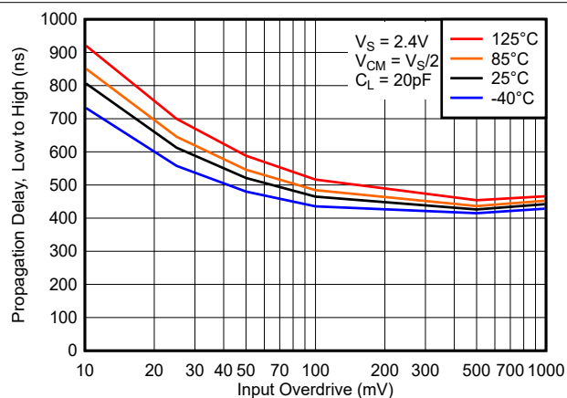
图 6-12. Propagation Delay, Low to High, 2.4V
