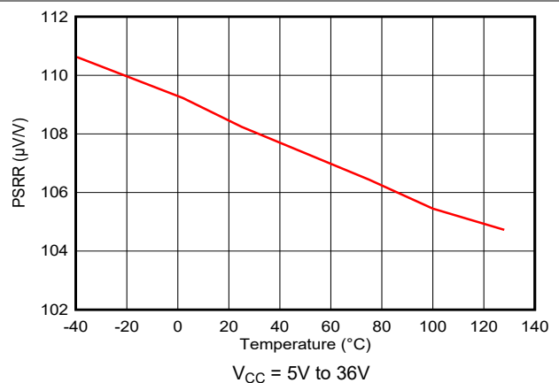
图 5-12. Supply-Voltage Rejection Ratio vs Temperature
