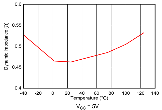
图 5-20. Reference Dynamic Impedance vs Temperature
