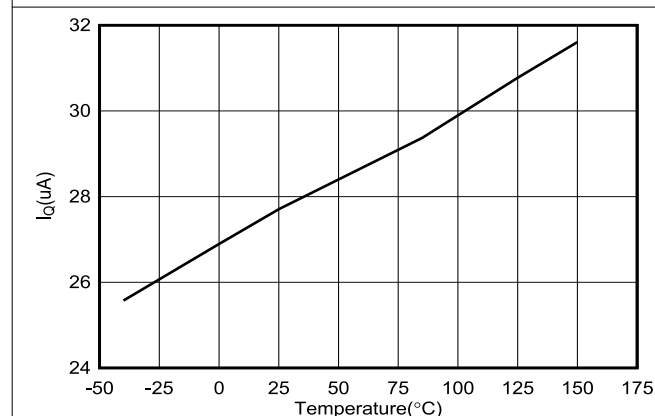
图 6-9. V_{IN} Quiescent Current Versus Temperature
