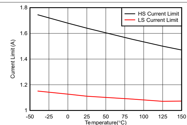
图 6-12. HS and LS Current Limit Versus Temperature
