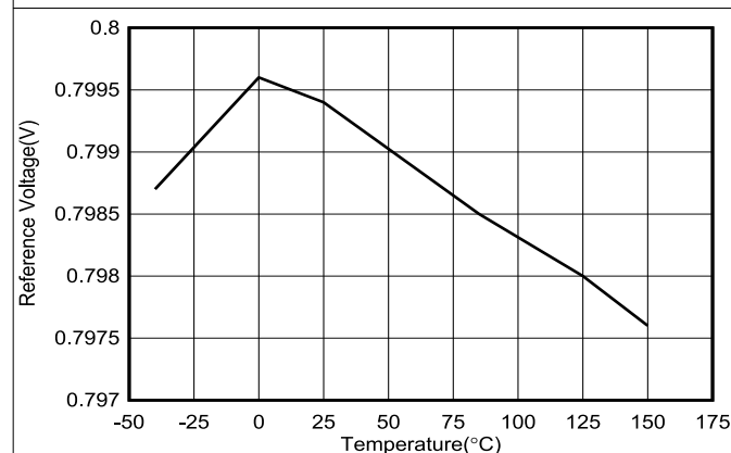
图 6-11. Reference Voltage Versus Temperature
