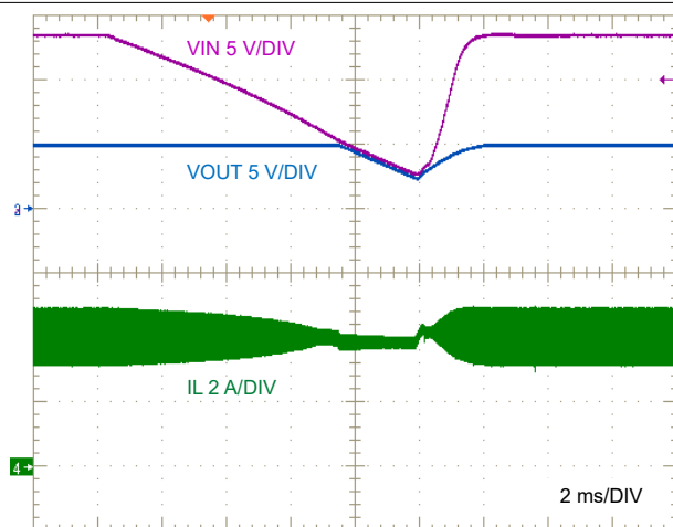
图 8-11. LM634x0-Q1 Line Transient and Recovery from Dropout
