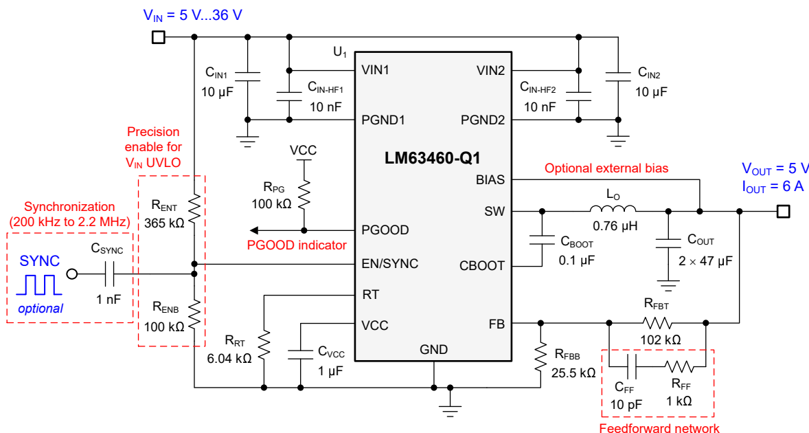
图 8-1. Application Circuit 1 - 5V, 6A at 2.1MHz
