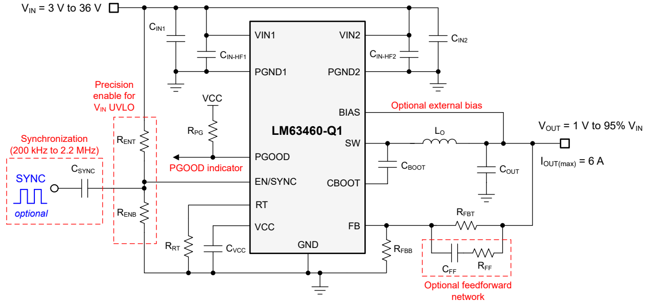
图 7-1. LM63460-Q1 Schematic Diagram with Input Voltage Operating Range of 3V to 36V
