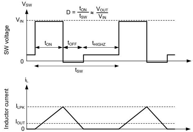
图 7-13. PFM Mode Operation at Light Loads
