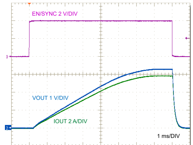
图 8-25. LM634x0-Q1 Enable On, Off, 6A Resistive Load
