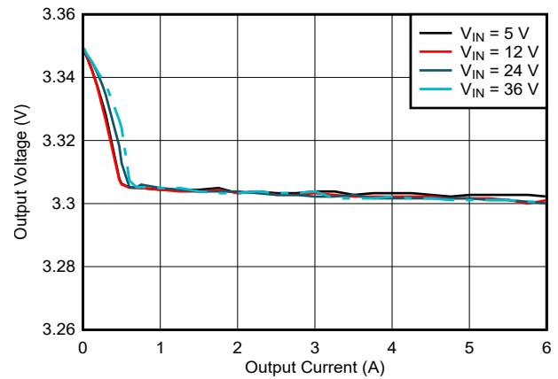
图 8-23. LM634x0-Q1 Load and Line Regulation
