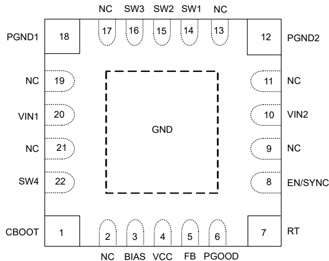
图 5-1. 22-Pin Enhanced HotRod™ QFN RYF Package (Top View)
