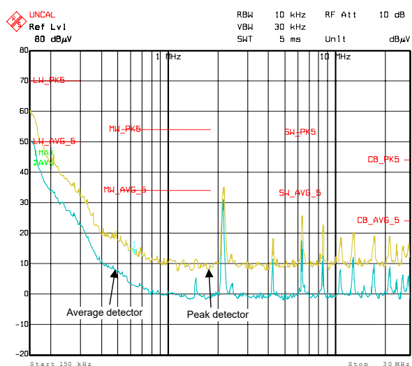
图 8-15. CISPR 25 Class 5 Conducted EMI, 150kHz to 30MHz
