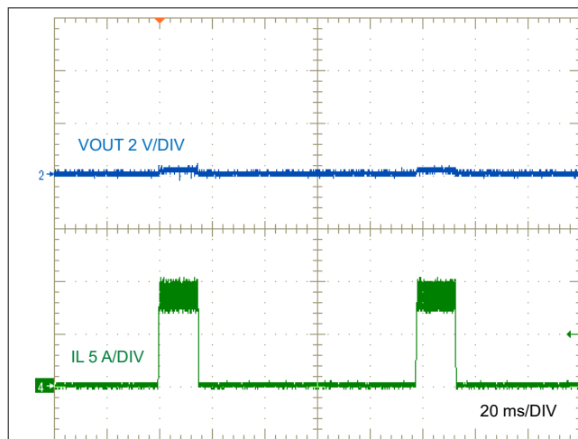
图 7-10. Inductor Current Bursts During Hiccup
