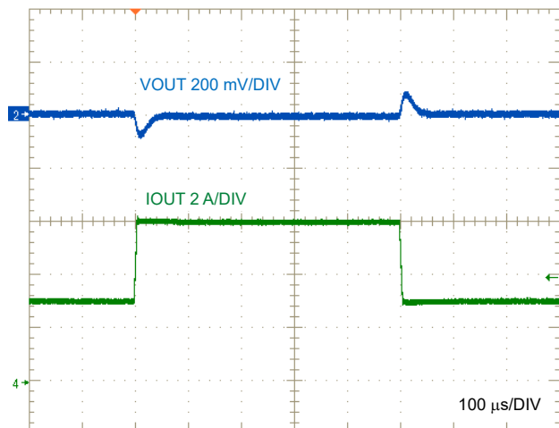
图 8-26. LM634x0-Q1 Load Transient, I_{OUT} = 3A to 6A
