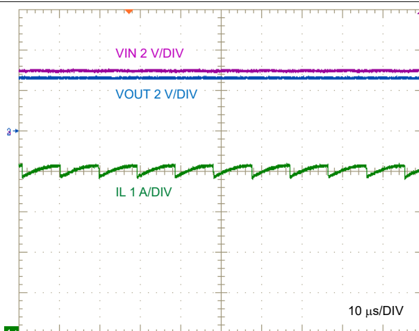
图 8-12. LM634x0-Q1 Frequency Foldback in Dropout, V_{IN} = 3V
