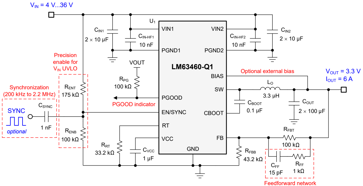
图 8-21. Application Circuit 3 - 3.3V, 6A at 400kHz
