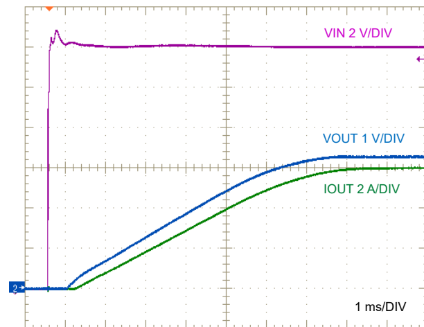
图 8-24. LM634x0-Q1 Start-Up, 6A Resistive Load
