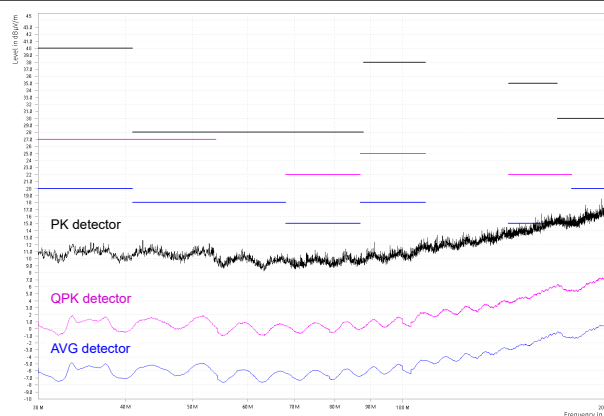
图 8-18. CISPR 25 Class 5 Radiated EMI, Bicon Antenna, Vertical Polarization, 30MHz to 200MHz
