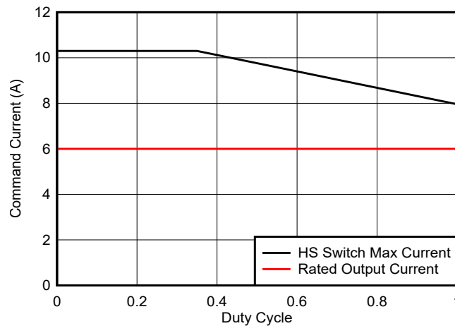
图 7-8. HS Switch Maximum Current as a Function of Duty Cycle for the LM63460-Q1
