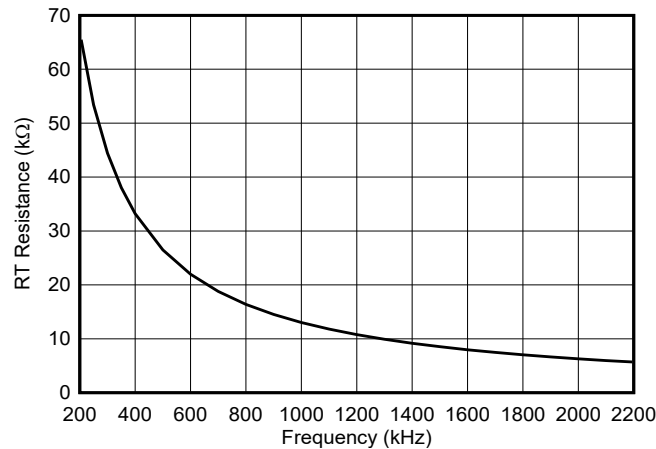
图 7-4. Setting the Switching Frequency
