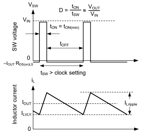
图 7-16. Valley Current Operation
