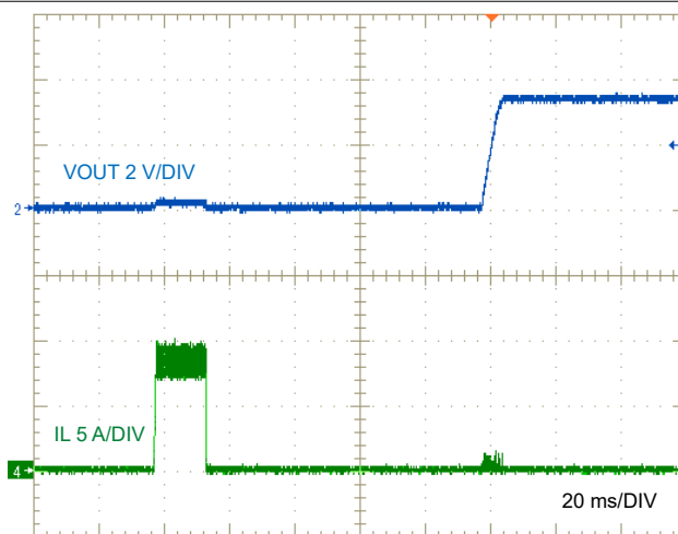
图 8-29. LM634x0-Q1 Short-Circuit Recovery to No Load
