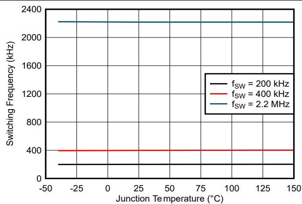
图 6-5. Switching Frequency Set by RT Resistor
