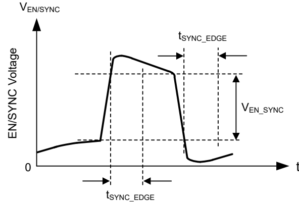
图 7-2. Typical Synchronization Waveform Applied to EN/SYNC
