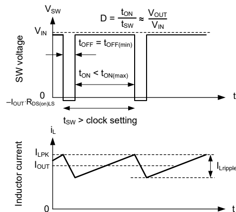
图 7-17. Switching Frequency and Output Voltage in Dropout
