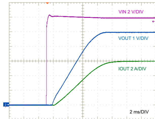
图 8-5. LM634x0-Q1 Start-Up, 6A Resistive Load
