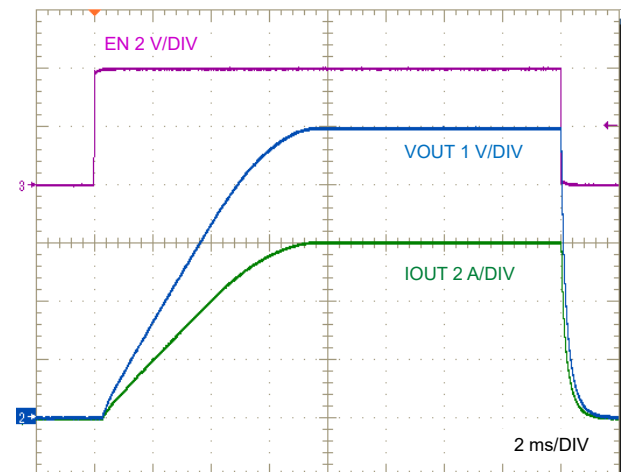
图 8-6. LM634x0-Q1 Enable On and Off, 6A Resistive Load
