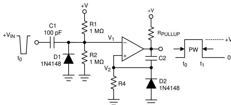
图 8-15. One-Shot Multivibrator
