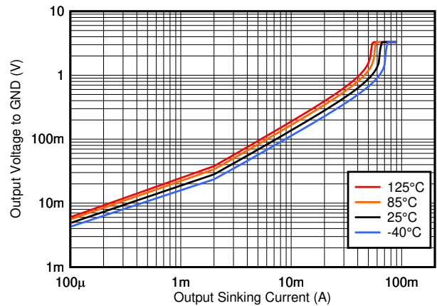
图 6-8. Output Sinking Current vs. Output Voltage, 3.3V
