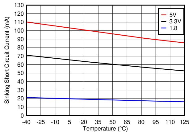
图 6-10. Sinking Short Circuit Current vs. Temperature
