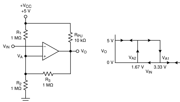
图 8-3. Inverting Configuration With Hysteresis
