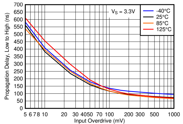
图 6-16. Propagation Delay, Low to High, 3.3V
