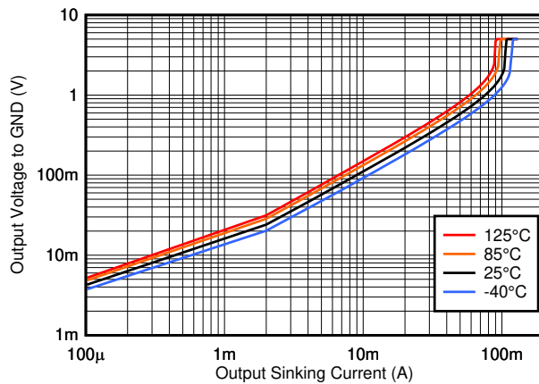
图 6-9. Output Sinking Current vs. Output Voltage, 5V
