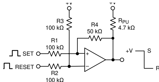
图 8-16. Bi-Stable Multivibrator
