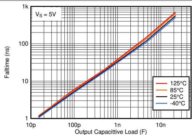
图 6-12. Fall time vs. Capacitive Load
