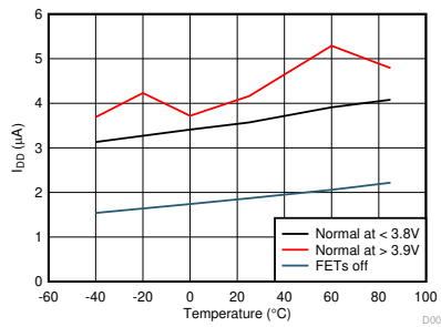
图 6-1. Normal and FET Off Current Across Temperature
