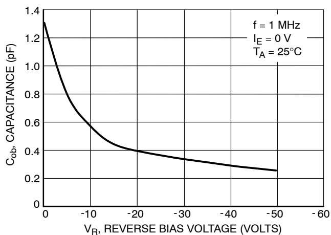
Figure 55. Output Capacitance
