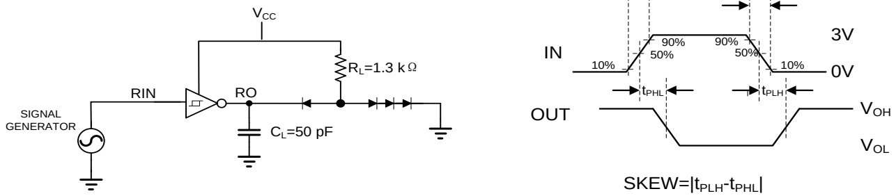
Figure 1 Receiver Propagation Delay and Receiver Skew
